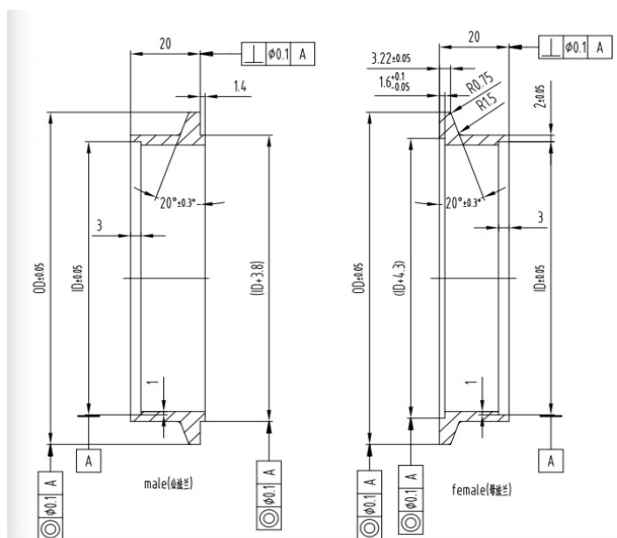
Flanges drawing:
